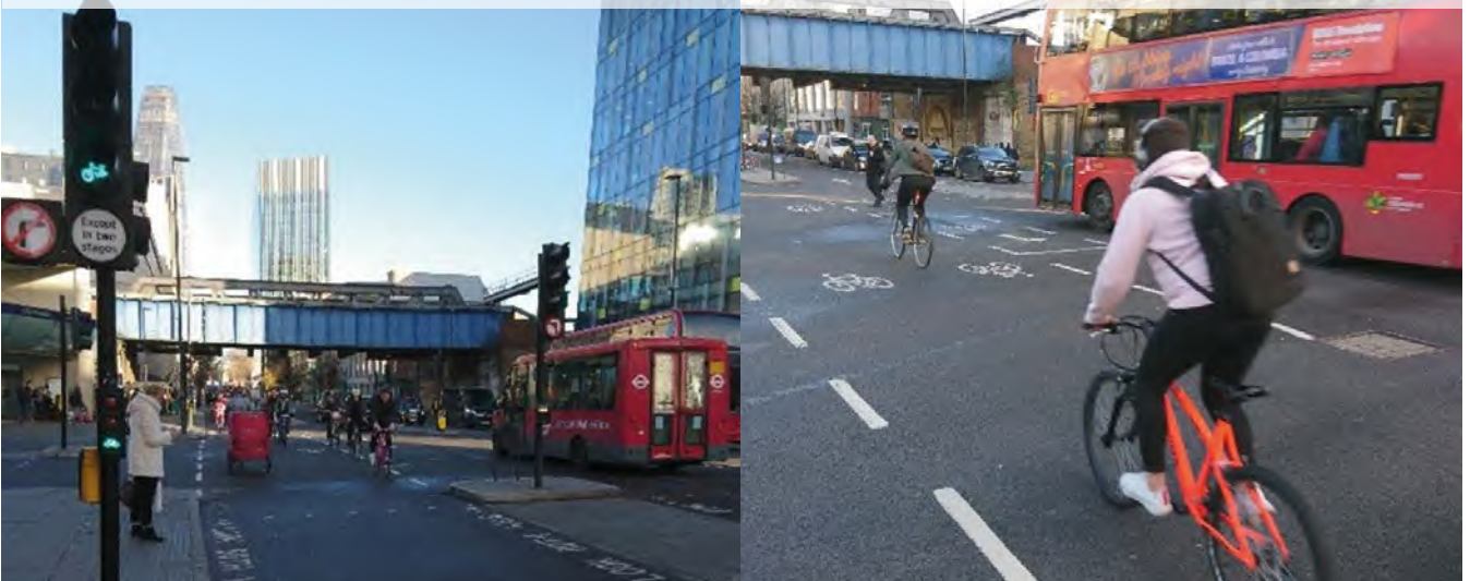
Figure 10.31: Signs and markings for two-stage turns from two-way cycle track, London
