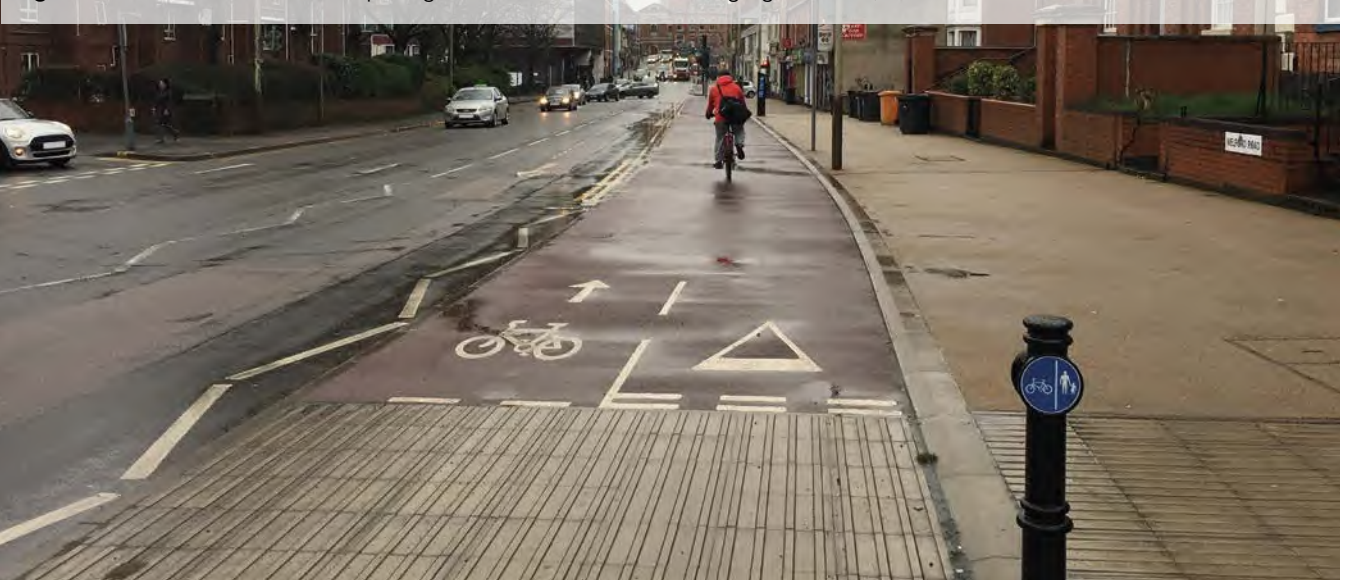
Figure 9.8: Correct use of tactile paving and low kerbs at start of segregated area, Leicester
